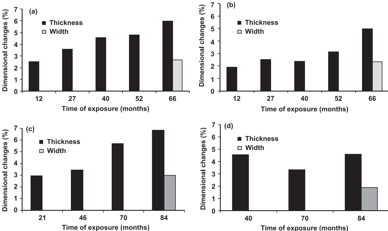
Figure 8.—Dimensional changes in wood–plastic composite #8 samples exposed at (a) the sunny location in Hilo, (b) the shadow location in Hilo, (c) the sunny location in Vancouver, and (d) the shadow location in Vancouver.
