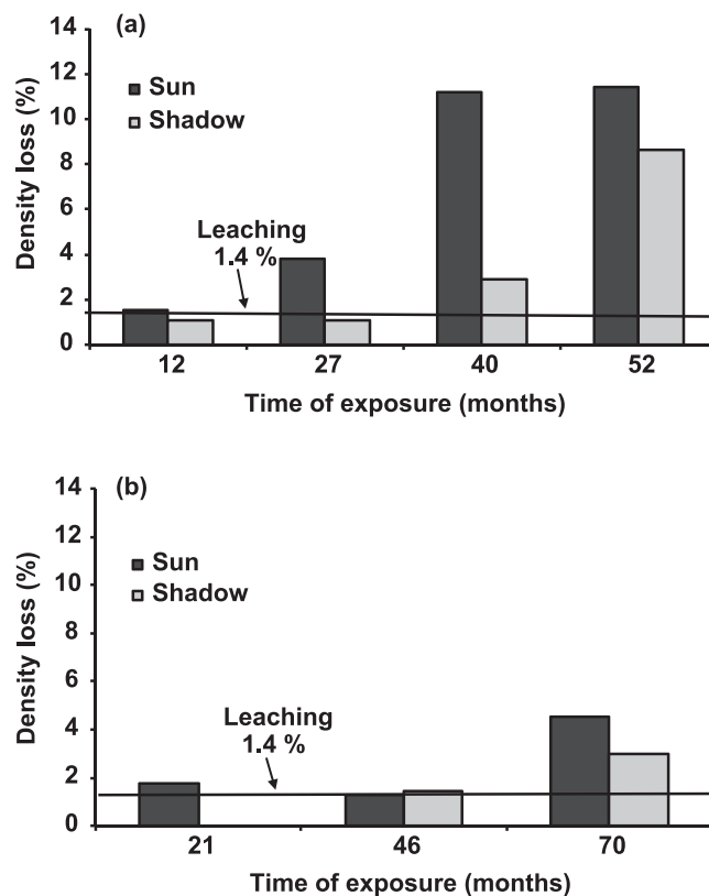
Figure 11.—Density loss from leaching and decay for wood–plastic composite sample #8 (a) exposed in Hilo and (b) exposed in Vancouver.
