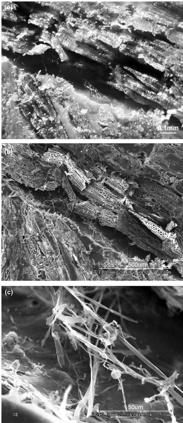
Figure 5.—Discolored cross section of wood–plastic composite #8 exposed at the sunny site in Hilo for 27 months. (a) Optical magnification of brown decayed wood particles with traces of white resin. (b) Scanning electron microscopy (SEM) image of the same area. (c) SEM image showing the magnified remains of decayed wood and fungal mycelia in the same area.
