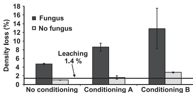
Figure 10.—Density loss from leaching and decay for wood–plastic composite #8 laboratory samples after soil block testing. The leaching value of 1.42 percent as calculated from field-exposed samples provides a baseline comparison for the soil block test results. Conditioning A = 2 weeks of soaking in water at room temperature; conditioning B = 5 days of soaking in water at 70°C.
